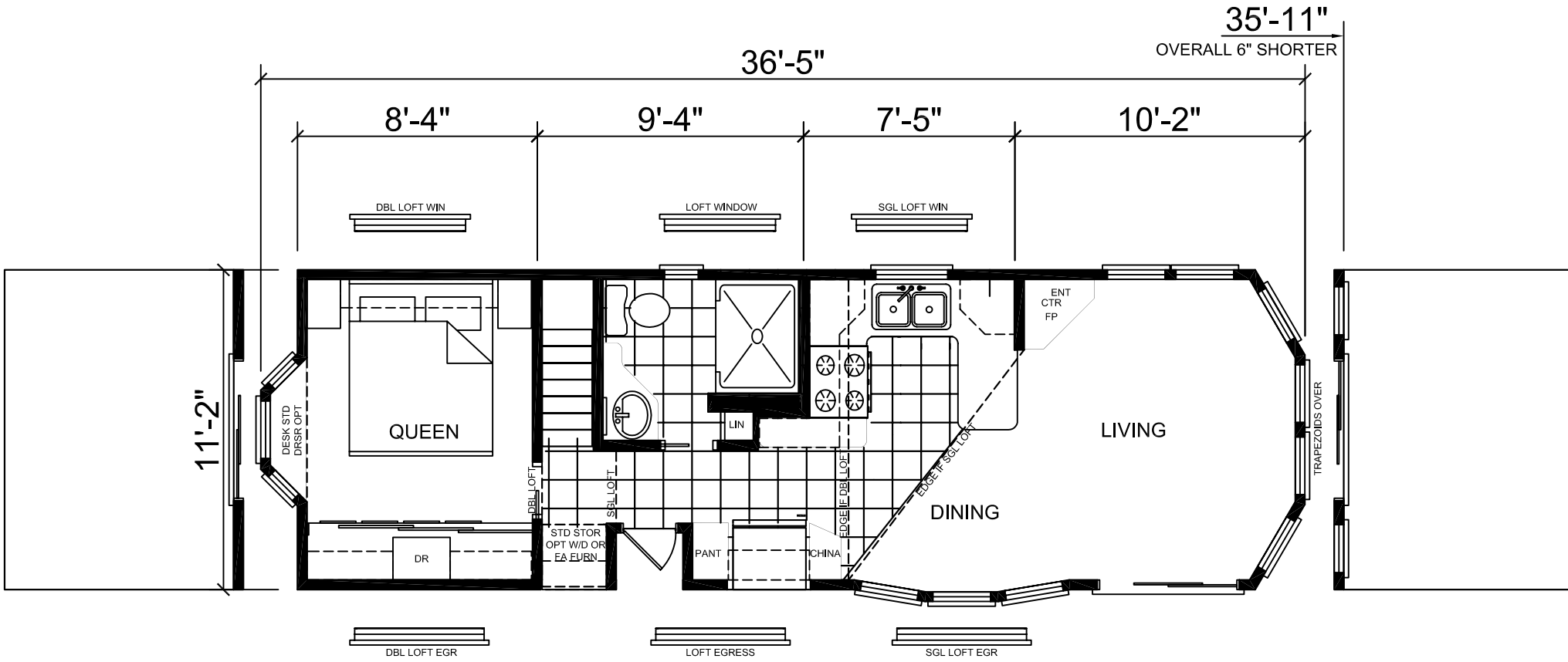
SINGLE AND DOUBLE LOFT OPTION
